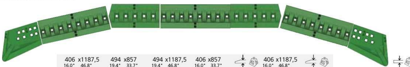
FULL U BLADE HEAVY DUTY & SUPER DOZER
